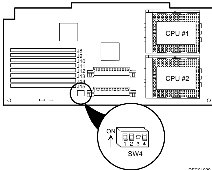
Figure 7. CPU Module Switch Location
